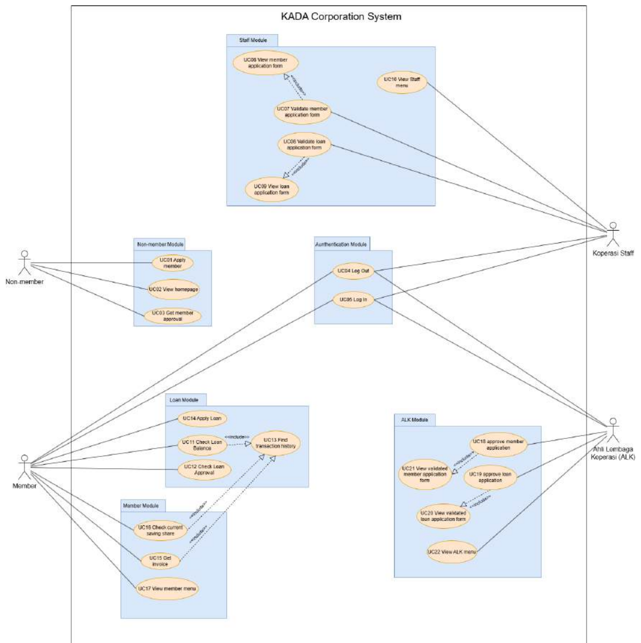
Figure 21: Use Case Diagram for KADA Corporation System
